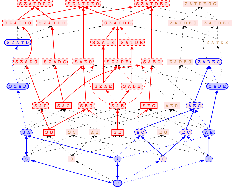
Figure 3: Decidability and complexity map of SCL sentence fragments. Round (blue) and square (red) nodes denote decidable and undecidable fragments, respectively. Solid borders on nodes correspond to theorems in this paper, while dashed ones are implied results. Directed edges indicate inclusion of fragments, while bidirectional ones denote polynomial-time reducibility. Solid edges are preferred derivations to obtain tight results from a complexity viewpoint, while dotted ones lead to worst upper-bounds or just model-theoretic properties. Finally, a light blue background indicates that the fragment enjoys the finite-model property, while those with a light red background do not satisfy such a property. Nothing is known for the ZATDE fragment reported in the figure. Letters denote the components of each given fragment: sequence (S), zero-or-one (Z), alternative (A) and transitive (T) paths; disjointness (D), order (O) and equality (E) of property pairs; cardinality constraints (C).
